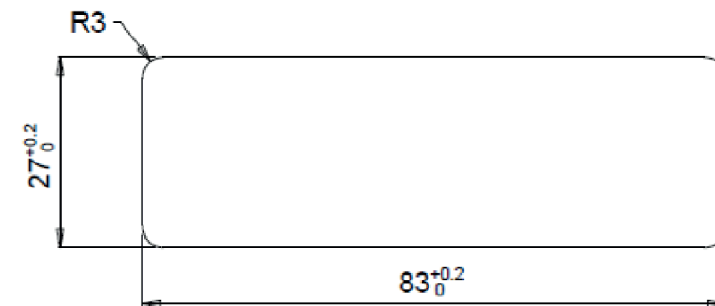
Flush mounting
