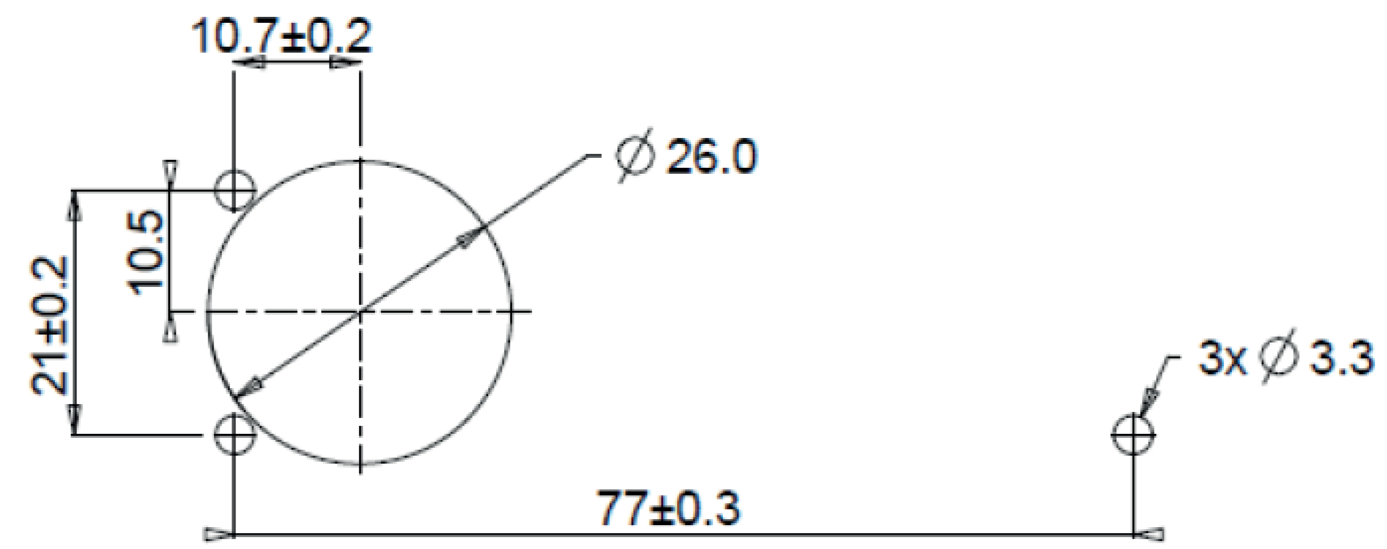
Surface mounting
