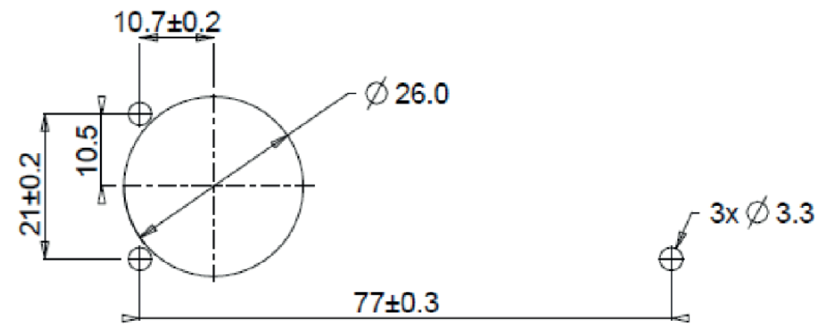
Surface mounting
