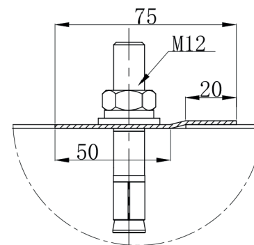
B Detail
