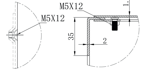
F Detail
