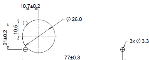
Surface mounting
